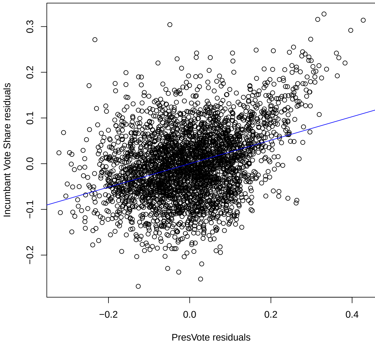
PresVote residuals vs Incumbant Vote Share residuals
