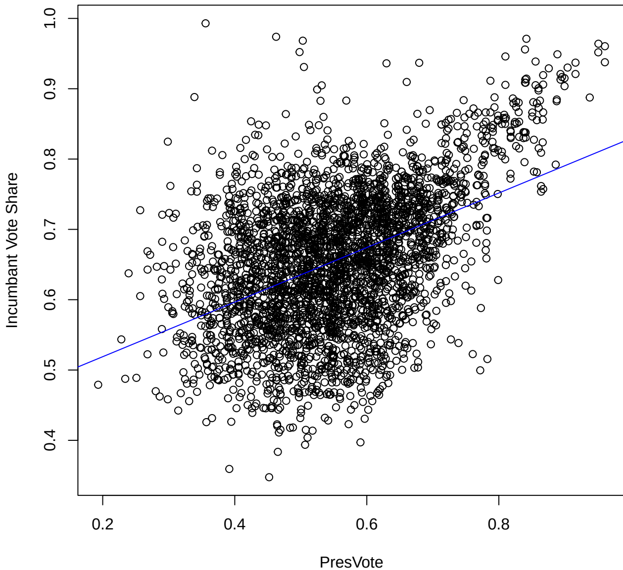
PresVote vs Incumbant Vote Share
