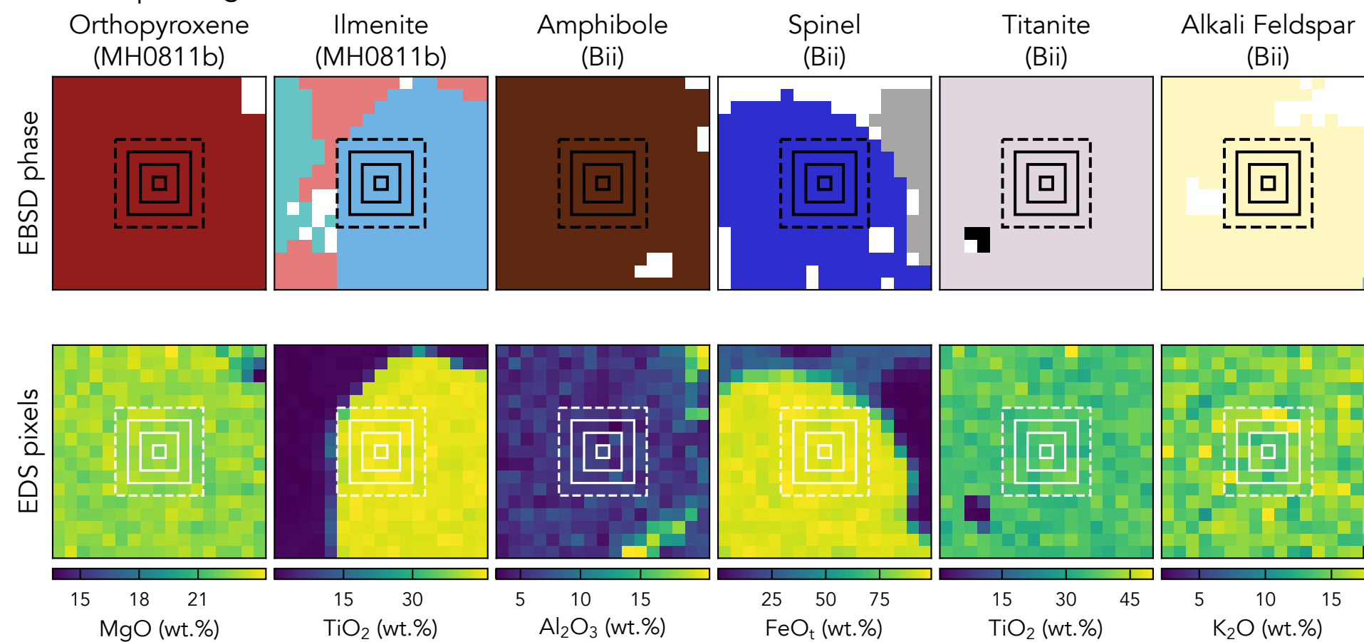
C. Example Regions: 1 \times 1 , 3 \times 3 and 5 \times 5 boxes
