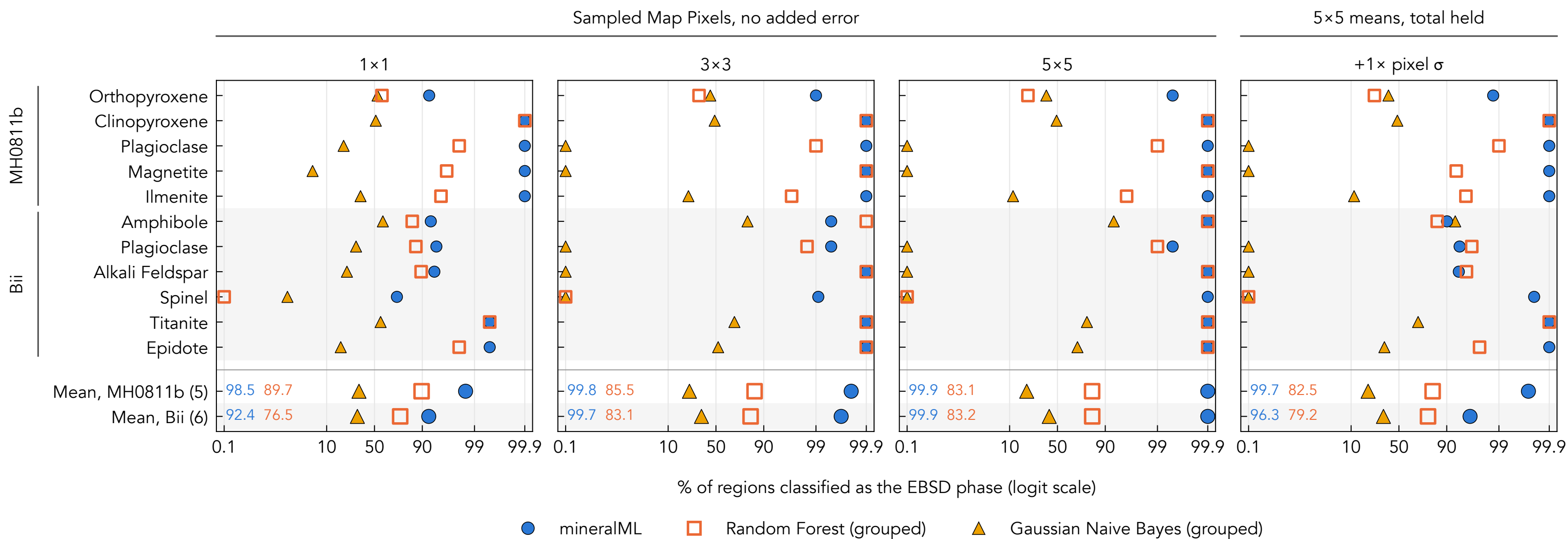
E. Classification of the sampled regions
