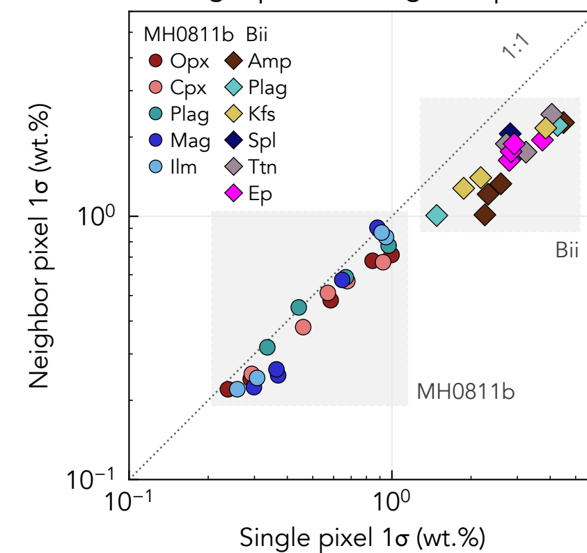
D. Single pixel vs neighbor pixel 1\sigma
