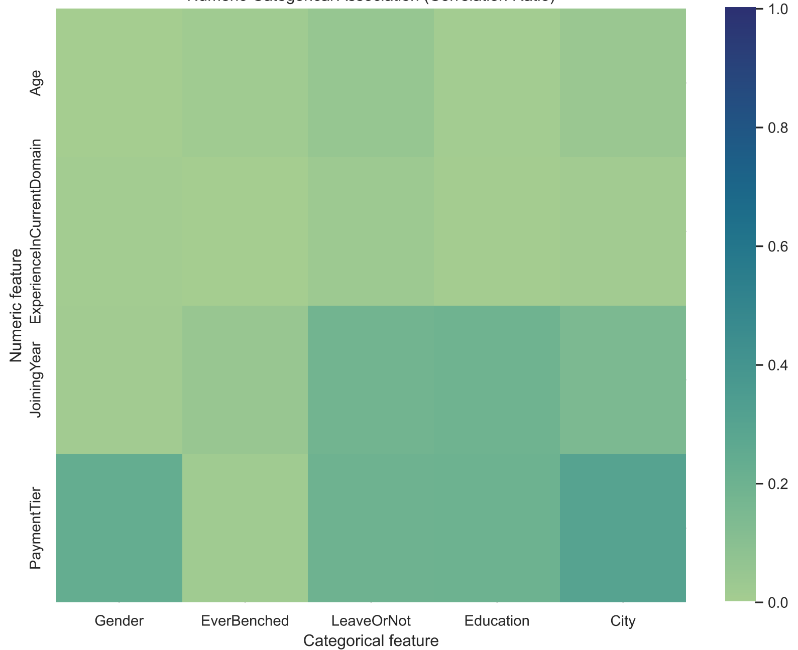
Numeric-Categorical Association (Correlation Ratio)
