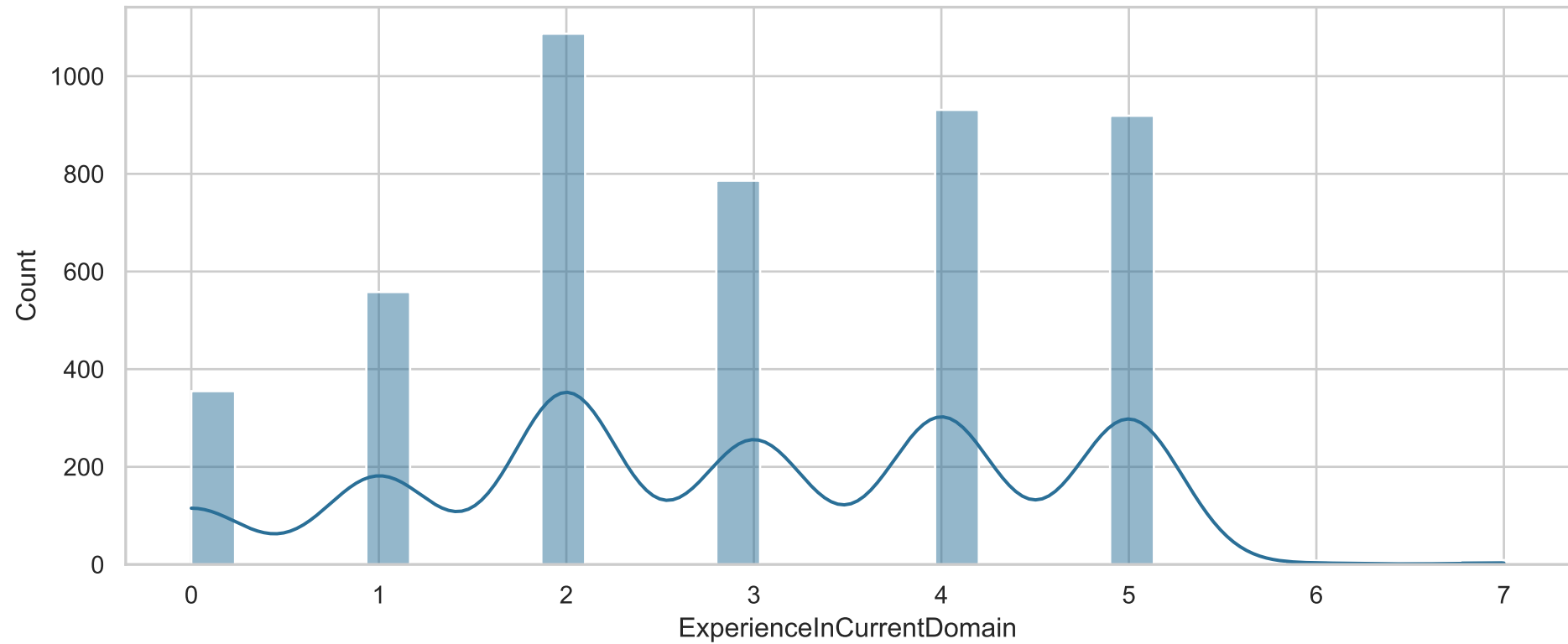
Distribution of ExperienceInCurrentDomain
