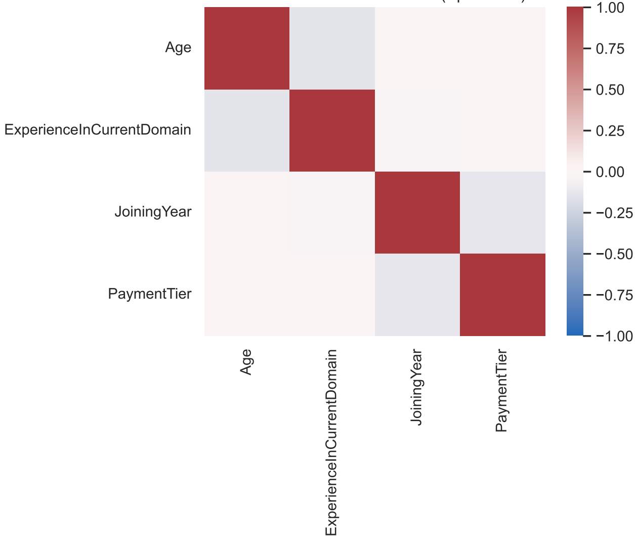
Numeric-Numeric Association (Spearman)
