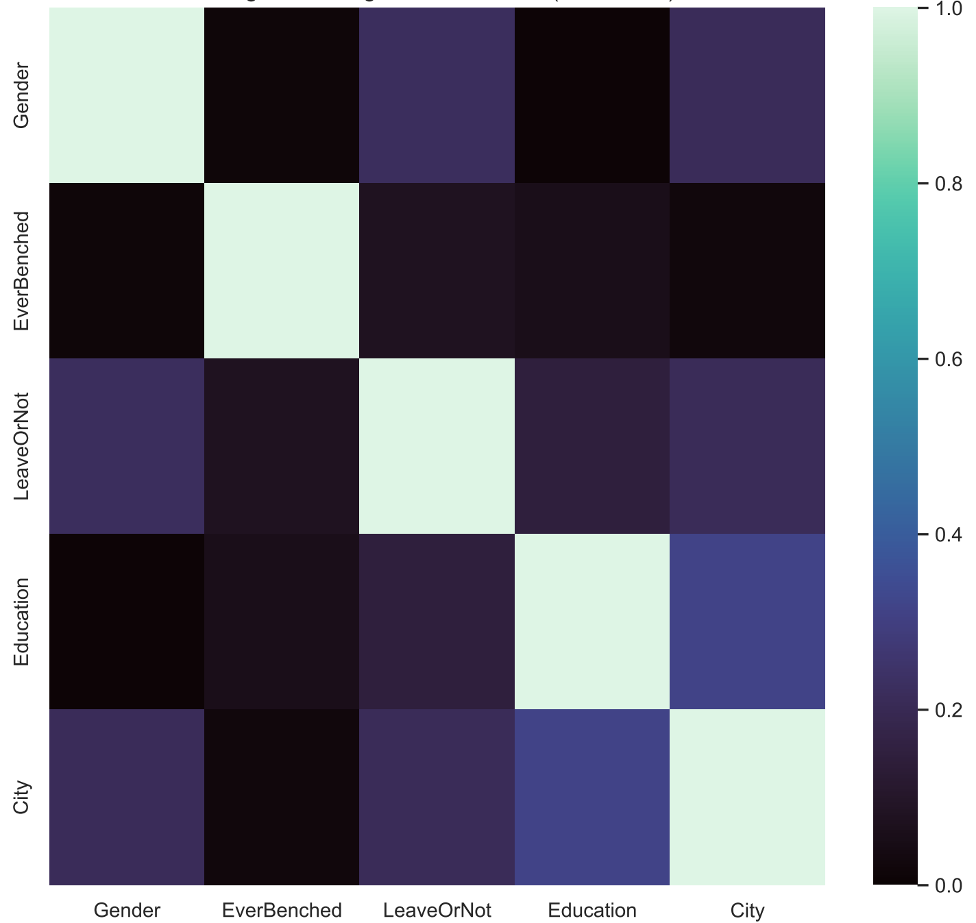
Categorical-Categorical Association (Cramer's V)
