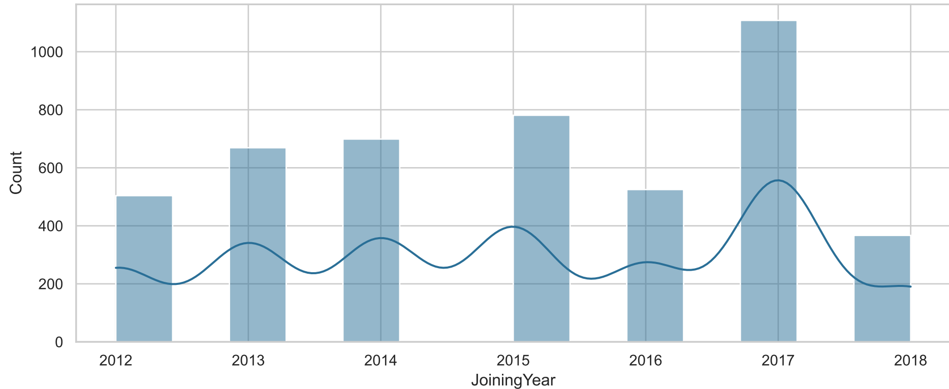
Distribution of JoiningYear
