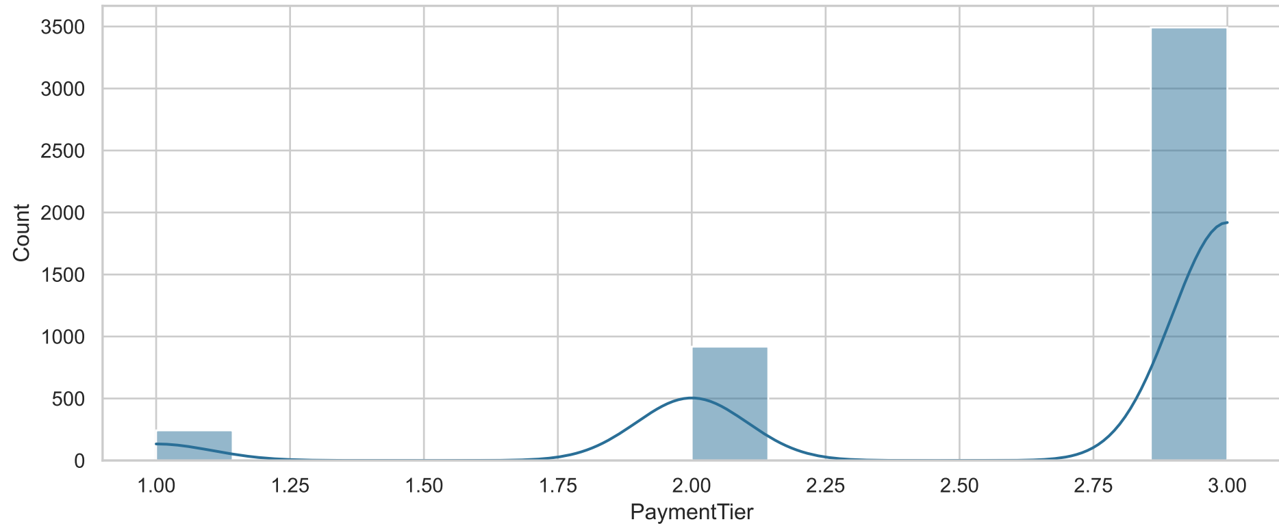
Distribution of PaymentTier
