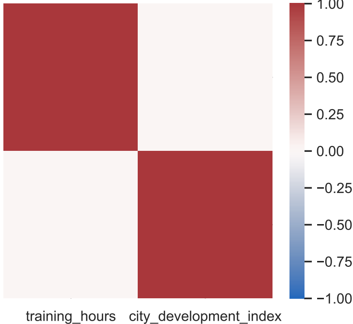
Numeric-Numeric Association (Spearman)
