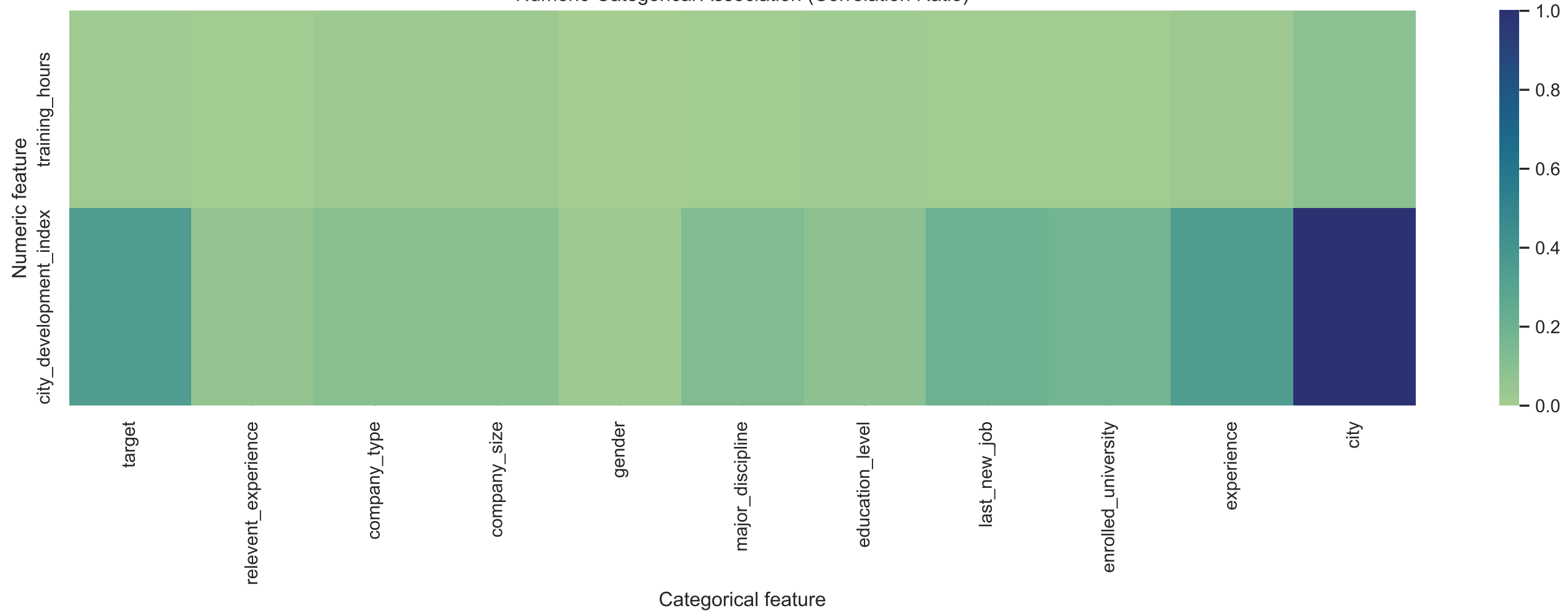
Numeric-Categorical Association (Correlation Ratio)
