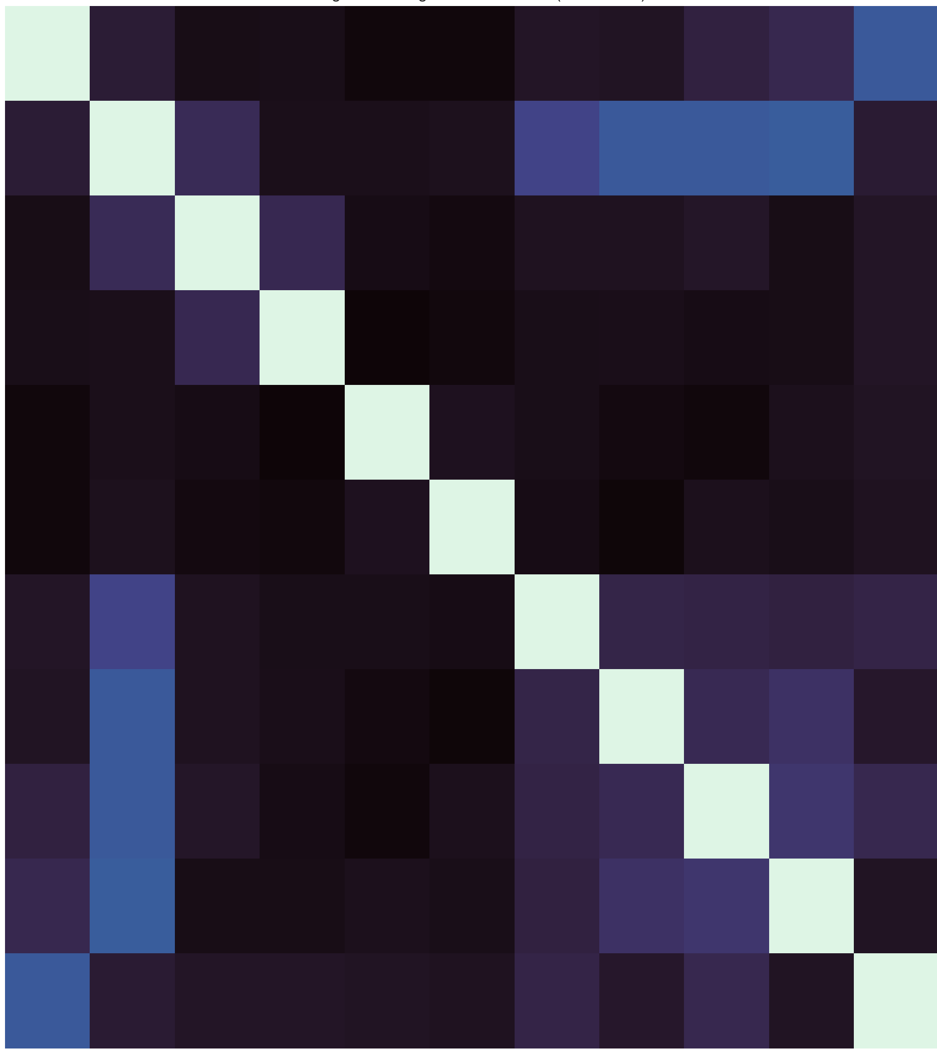
Categorical-Categorical Association (Cramer's V)
