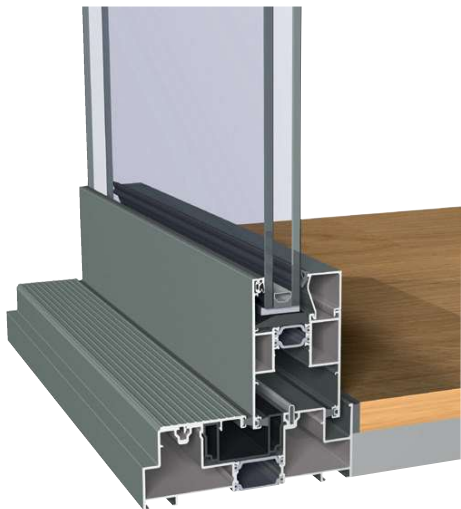
Flush floor detail
