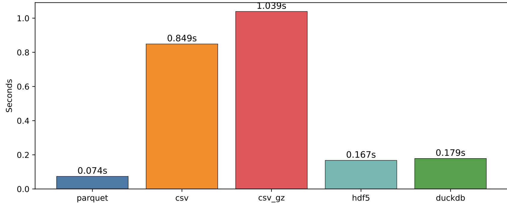
Read Time into Pandas DataFrame
