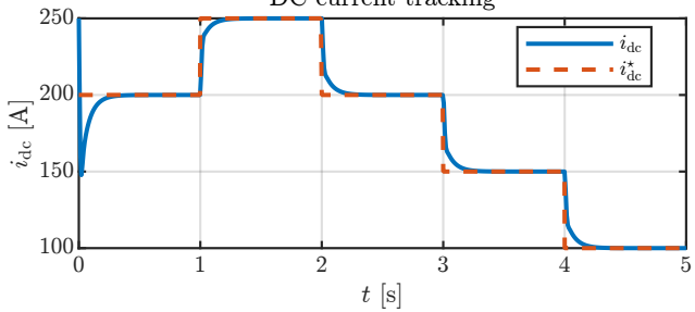
DC current tracking
