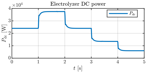
Electrolyzer DC power
