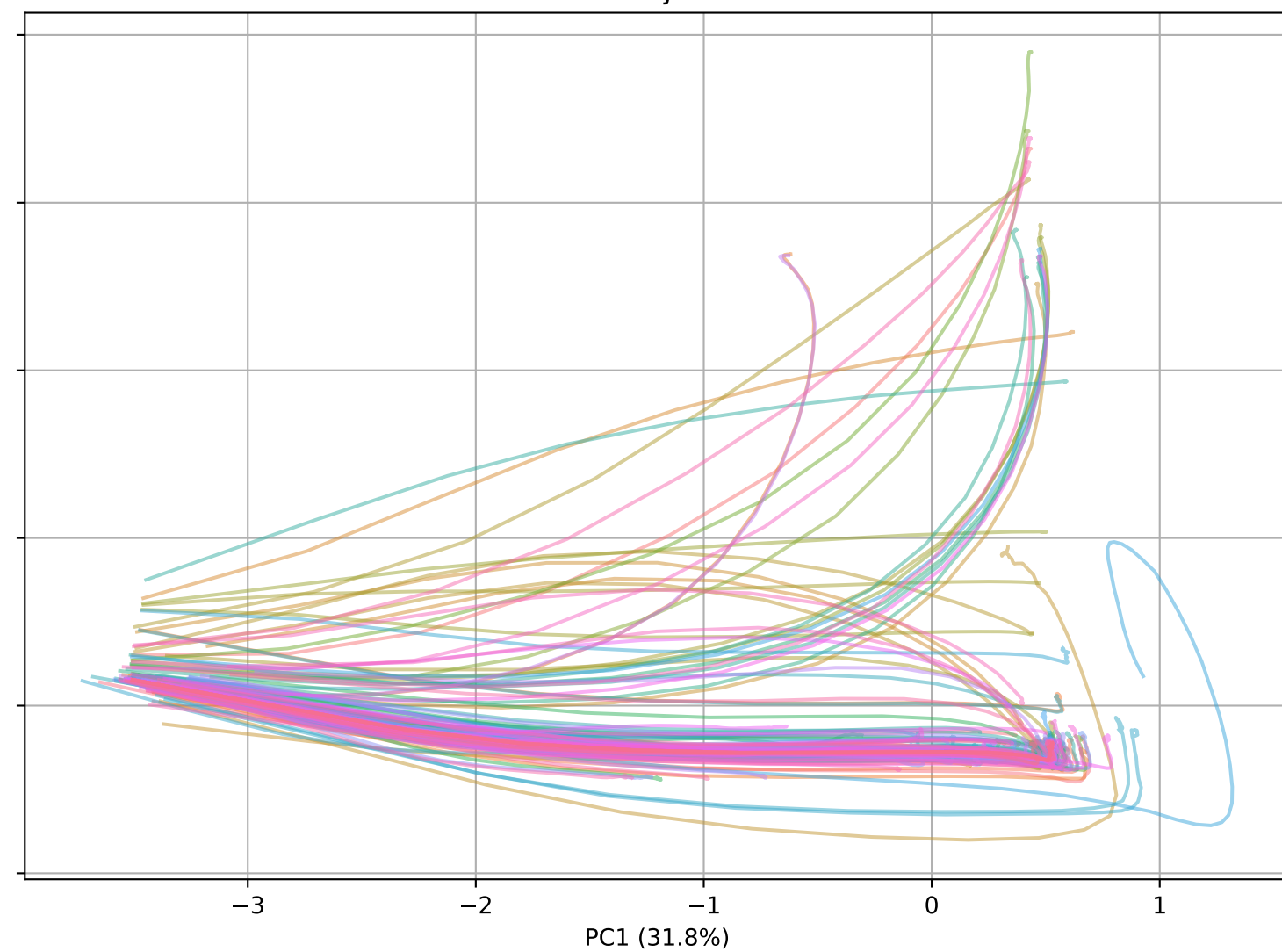
Model trajectories
