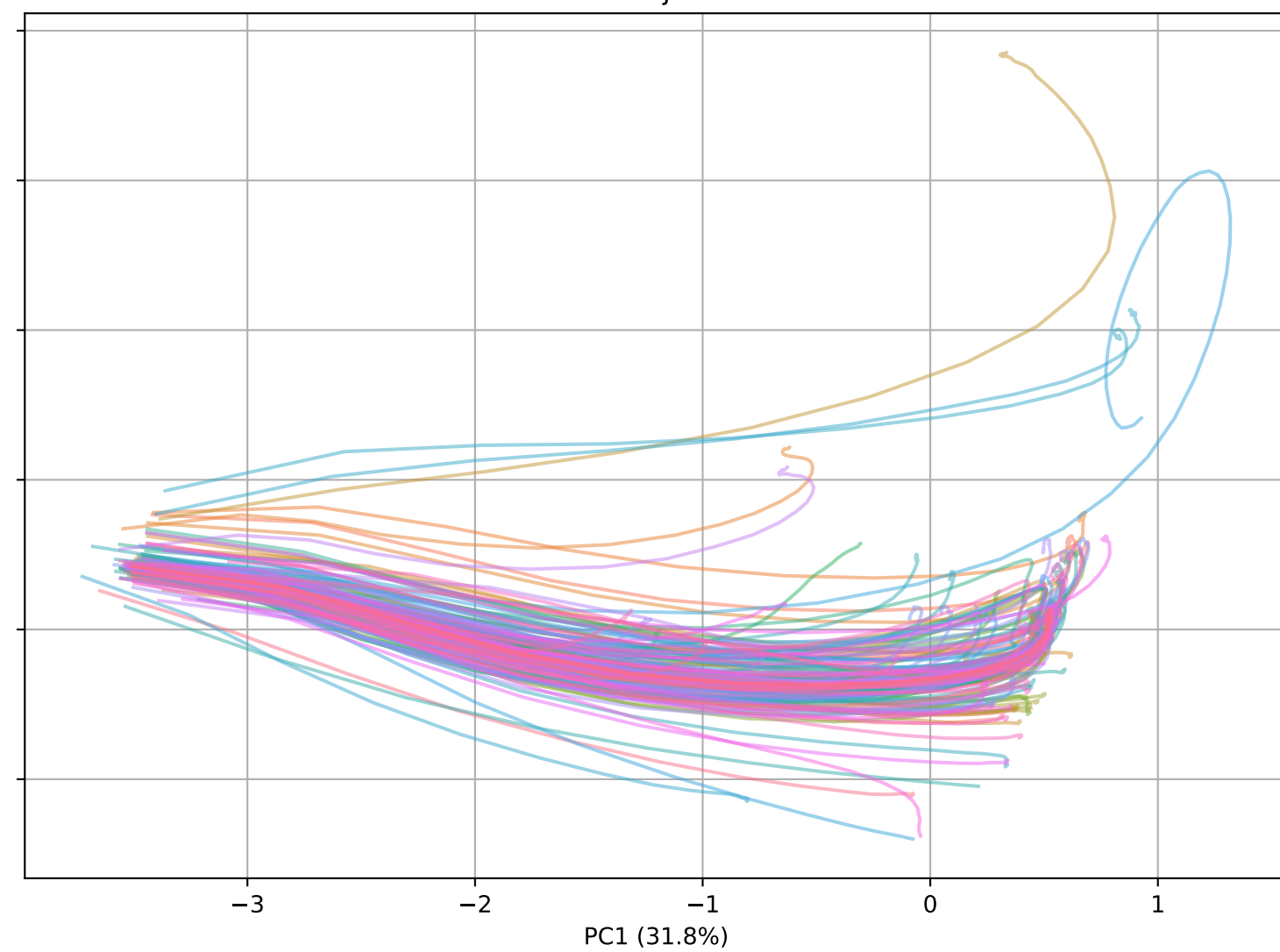
Model trajectories
