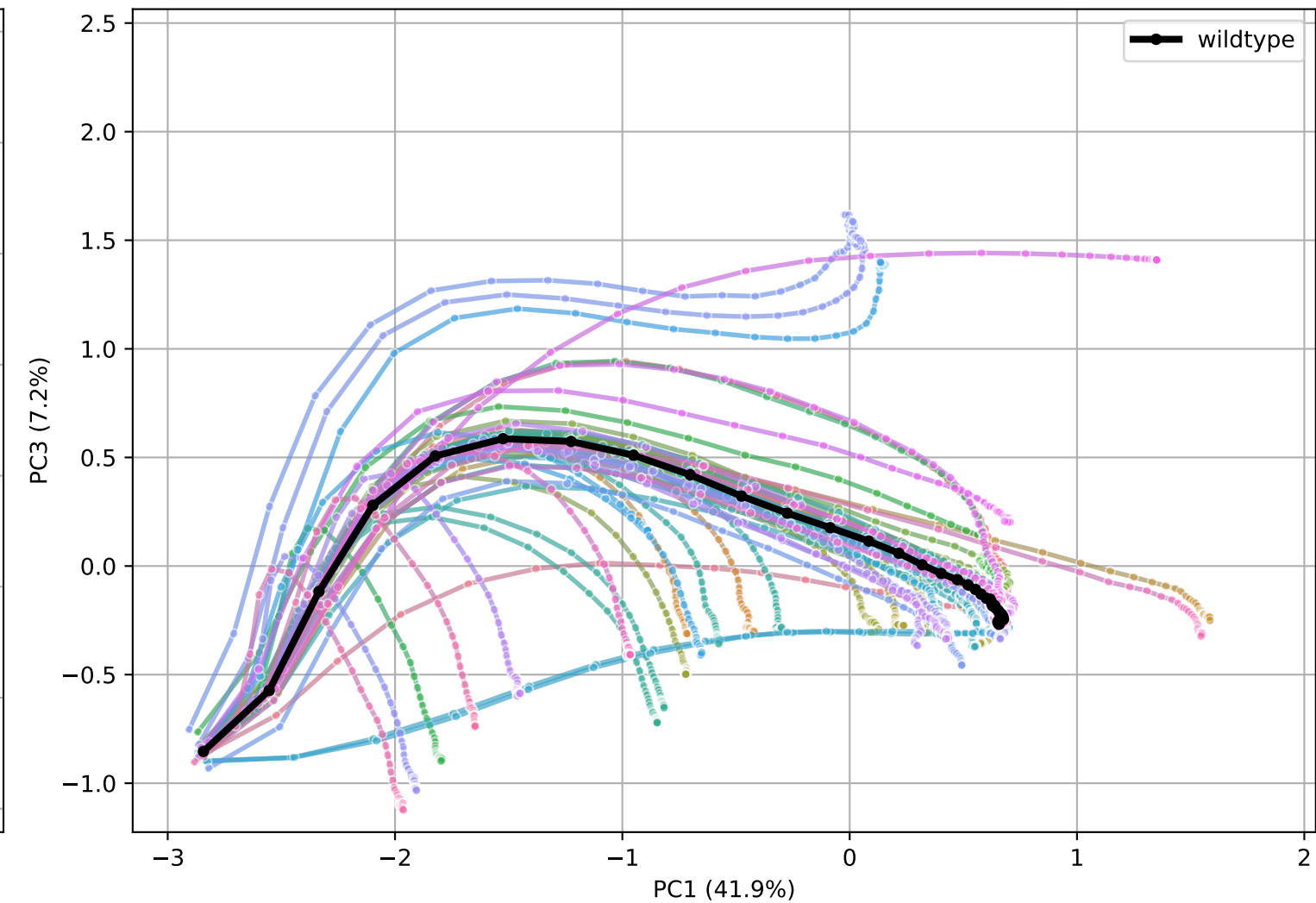
OFF perturbations + wildtype (n=109)
