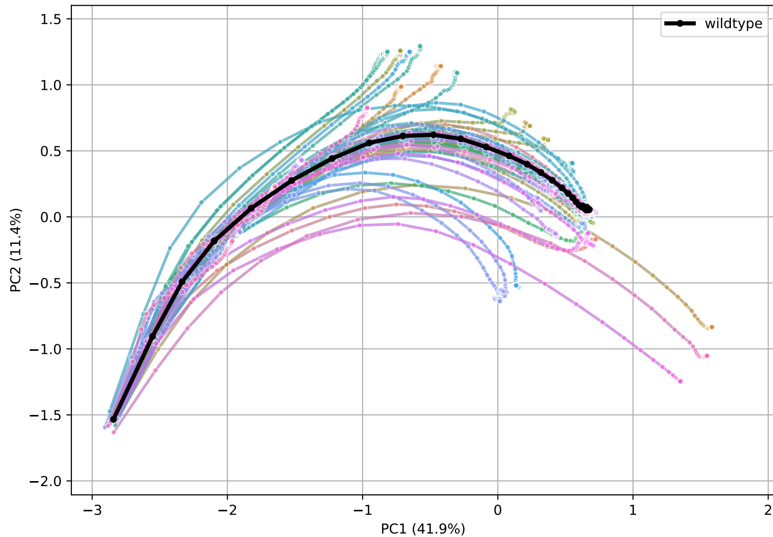
OFF perturbations + wildtype (n=109)
