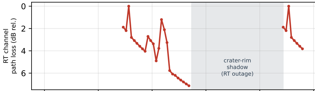
Closed loop: Sionna-RT lunar channel (real LOLA terrain) → live srsRAN
