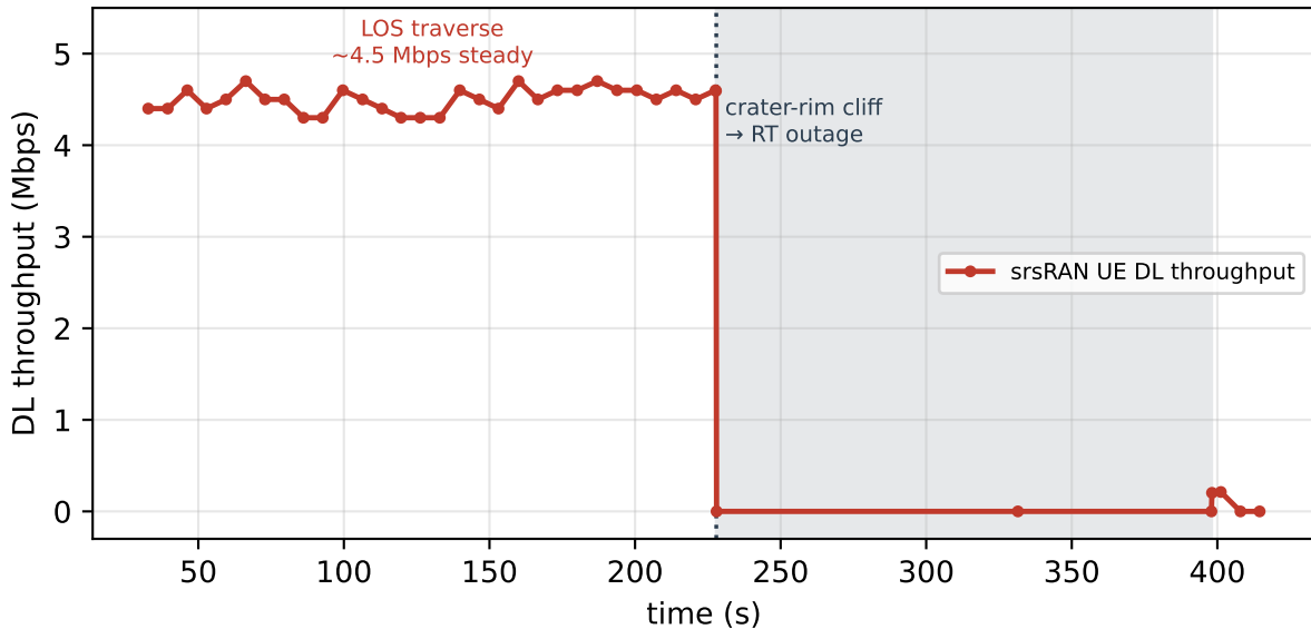
Closed loop: Sionna-RT lunar channel (real LOLA) → live srsRAN throughput
