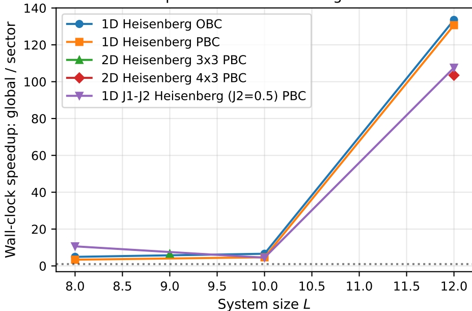
Sector decomposition is faster than global verification
