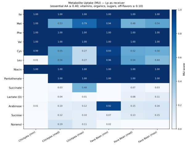
Fig. 1. MUP scores for L. plantarum as receiver across six legume medium scenarios. Values represent the fraction of feasible solutions requiring uptake of each metabolite. Empty cells indicate MUP below threshold or metabolite absent from that scenario.
