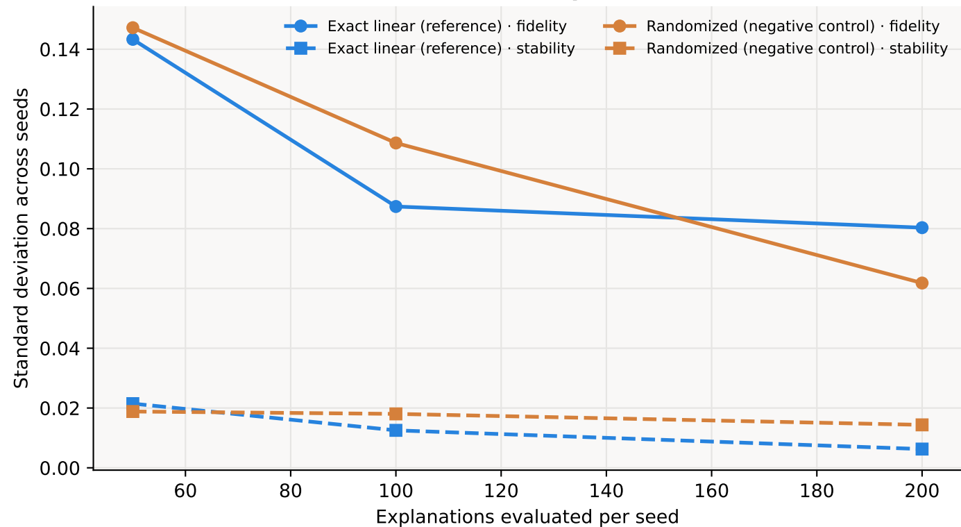
Variance decreases as evaluation sample size increases
