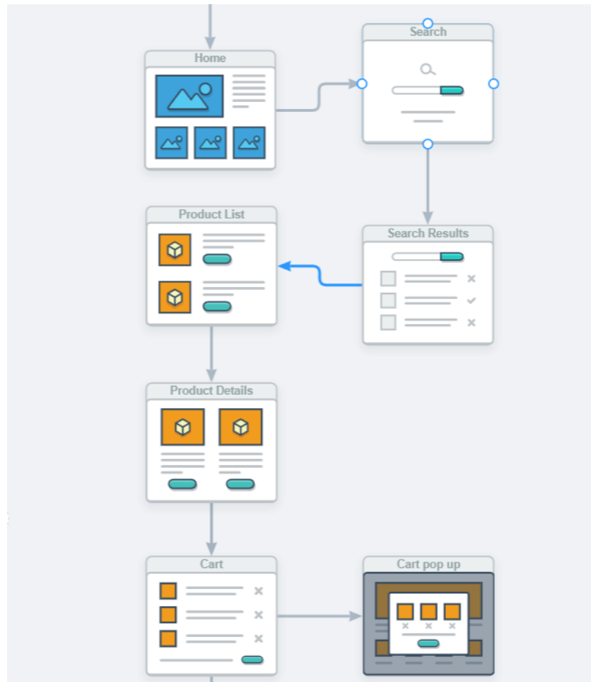
Fig 2: Search and Add to Cart — Home → Search → Results → Product → Cart
