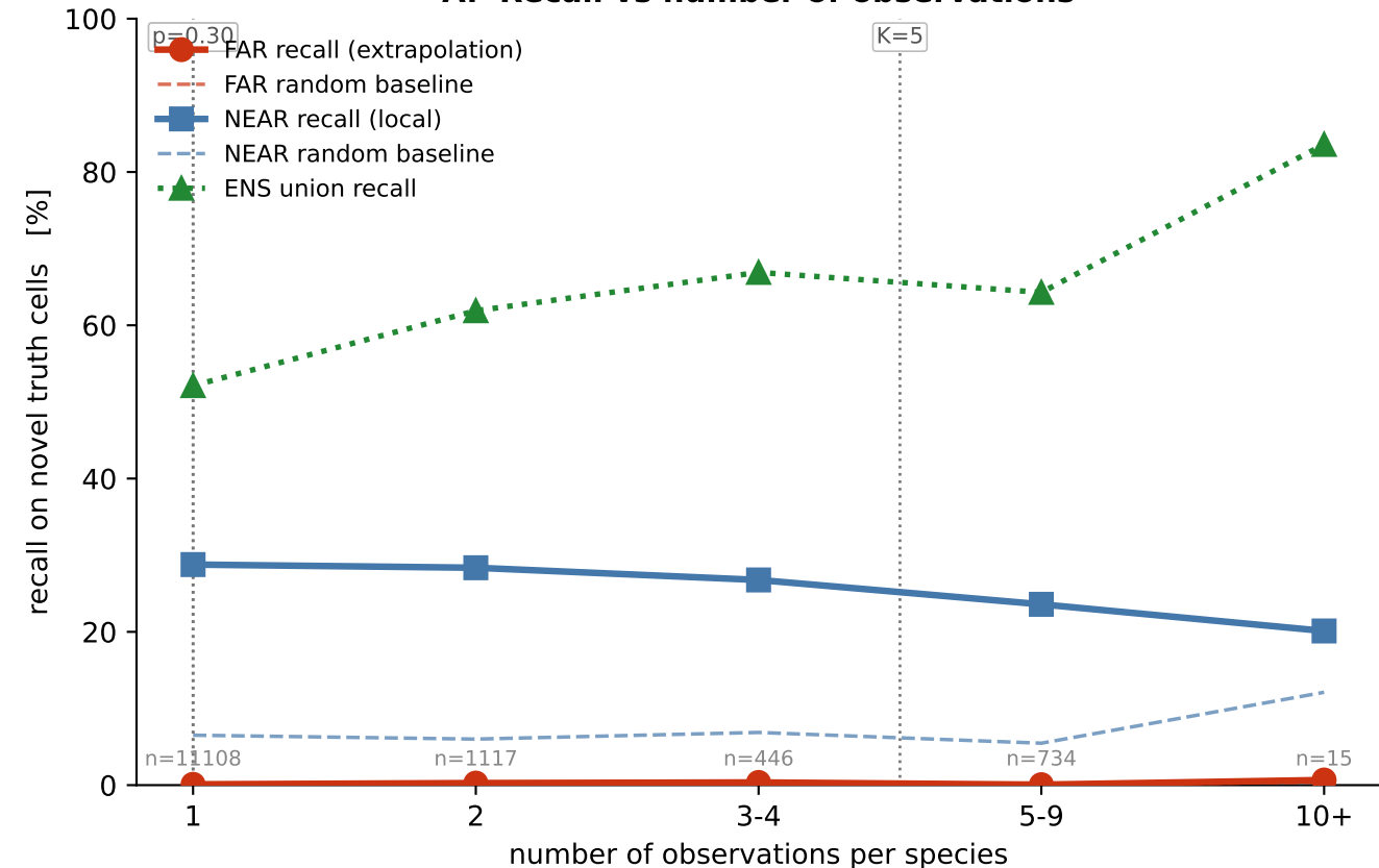
A. Recall vs number of observations
