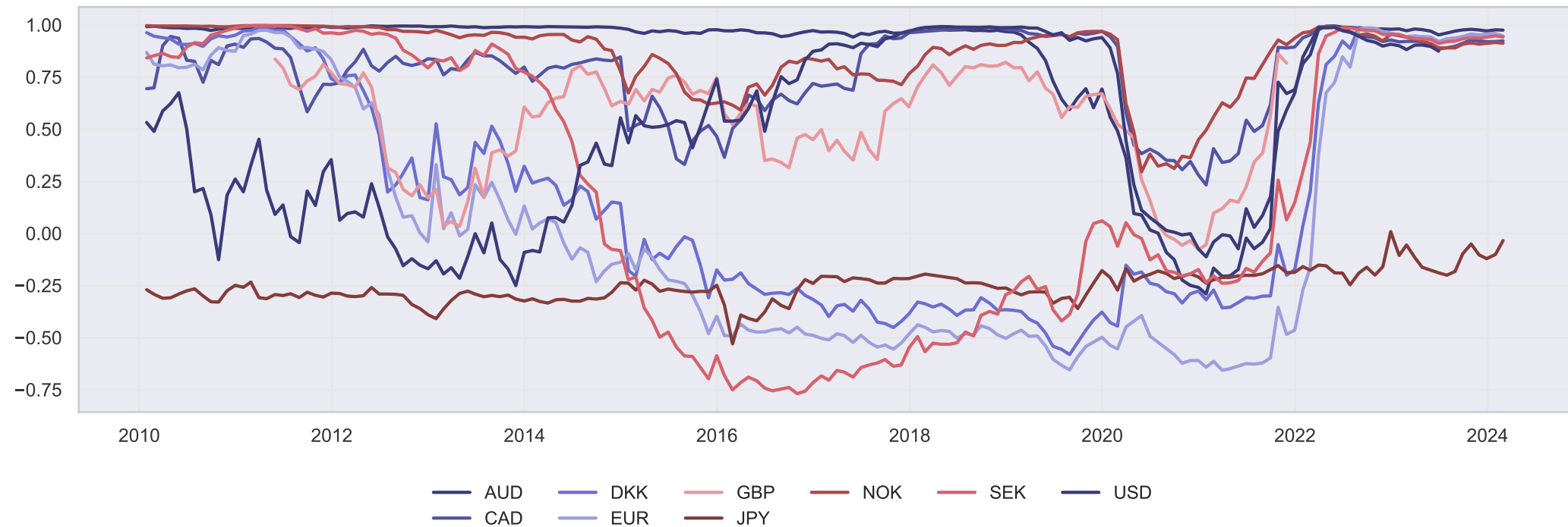
Correlation rho23
