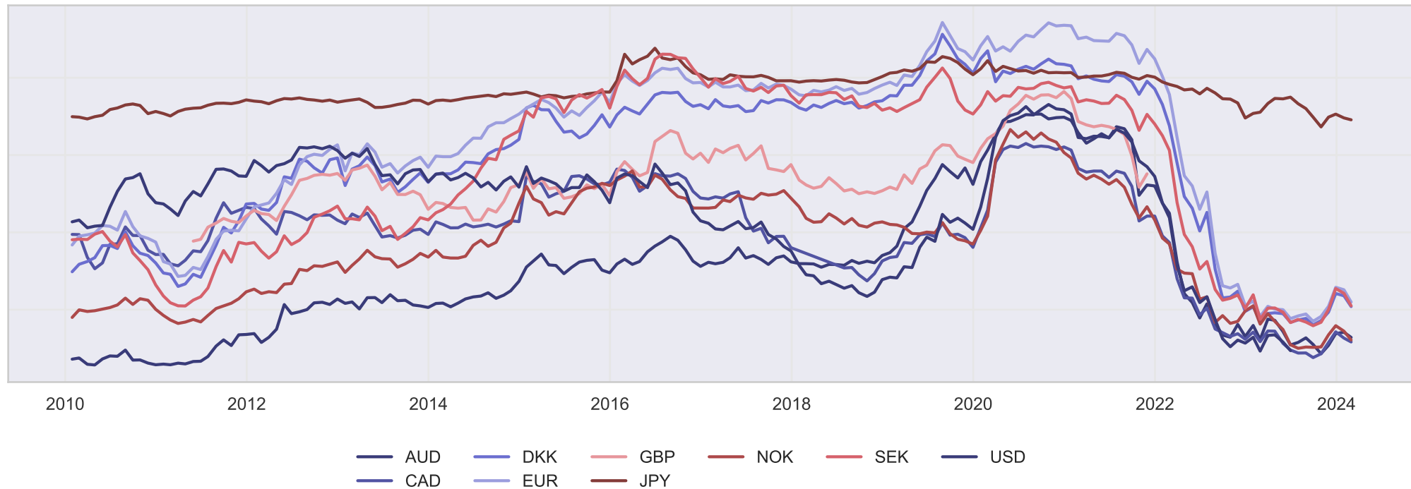
Volatility sigma2(z)
