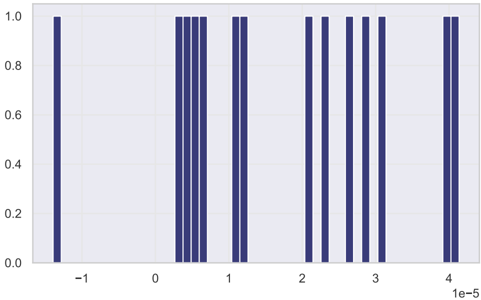
Histogram of rho13
