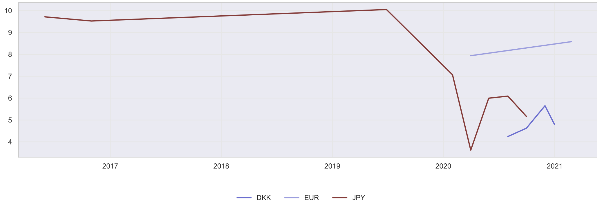
Volatility \sigma^2(z)
