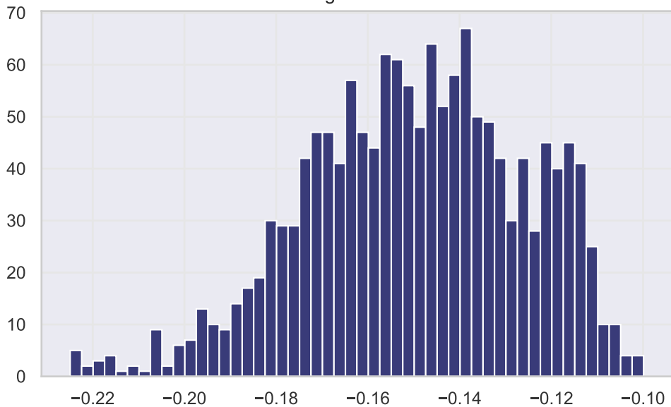
Histogram of \mu_1
