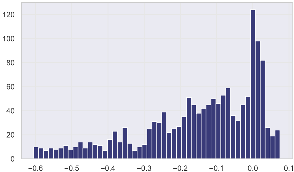
Histogram of rho12
