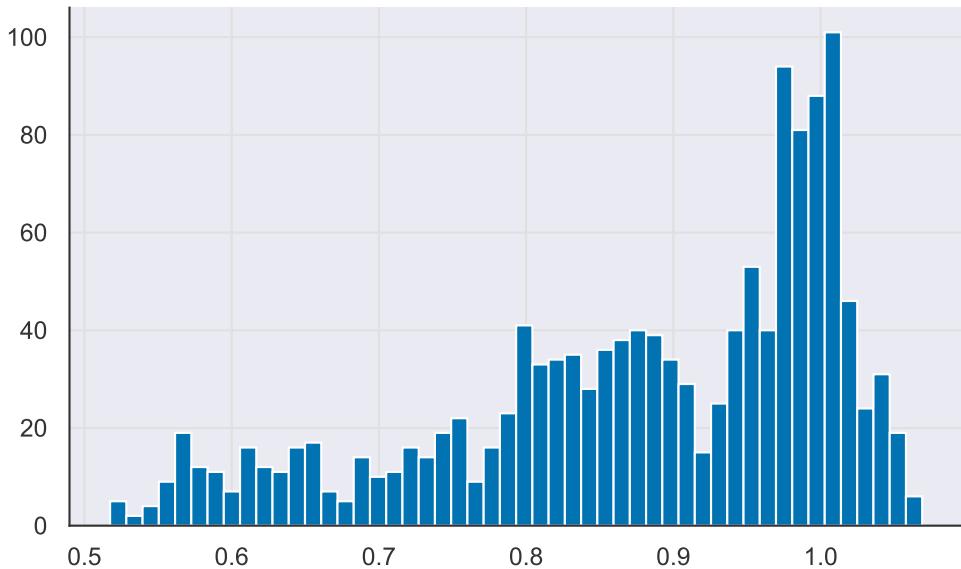
Histogram of sigma2
