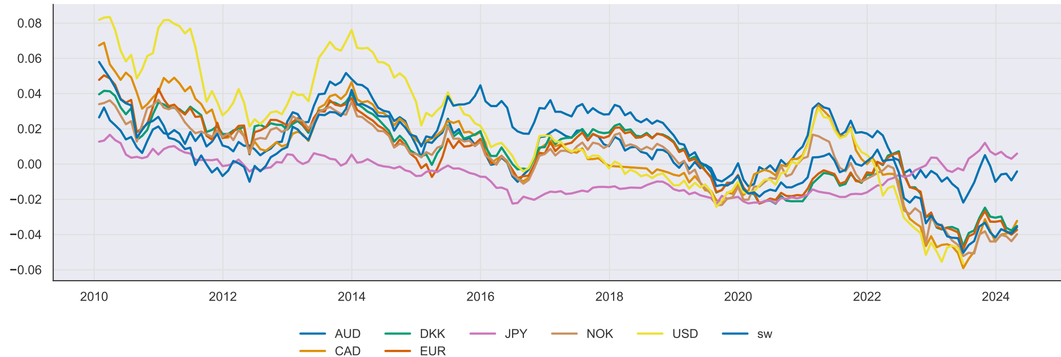
Drift \mu_1(z)
