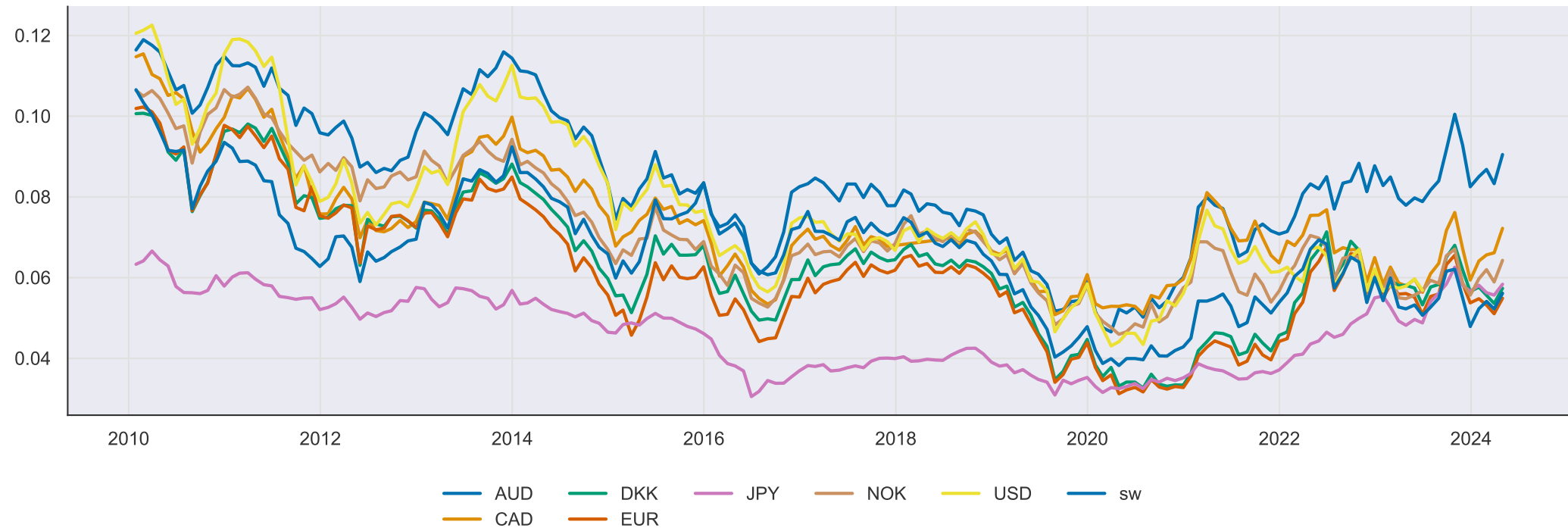
Drift \mu_2(z)
