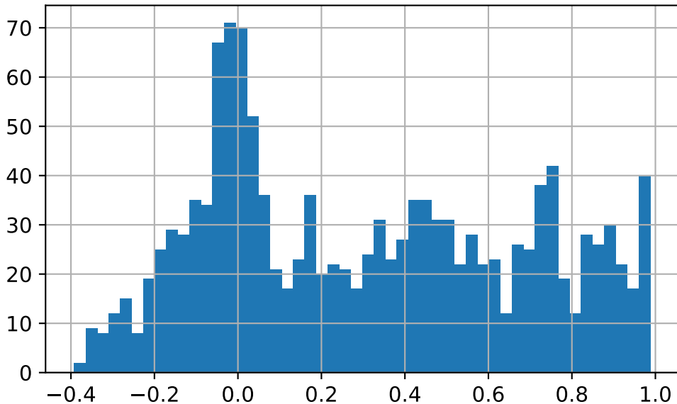
Histogram of rho
