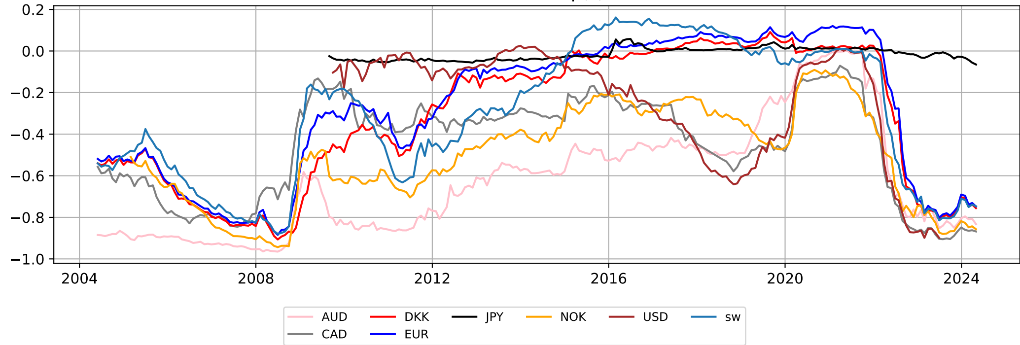
Correlation \rho(z)
