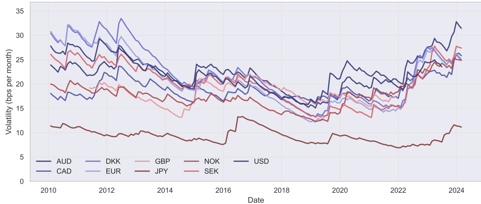
EWMA volatility — 30Y swap
