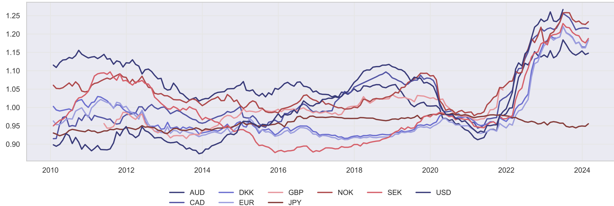
Volatility \sigma_3(z)
