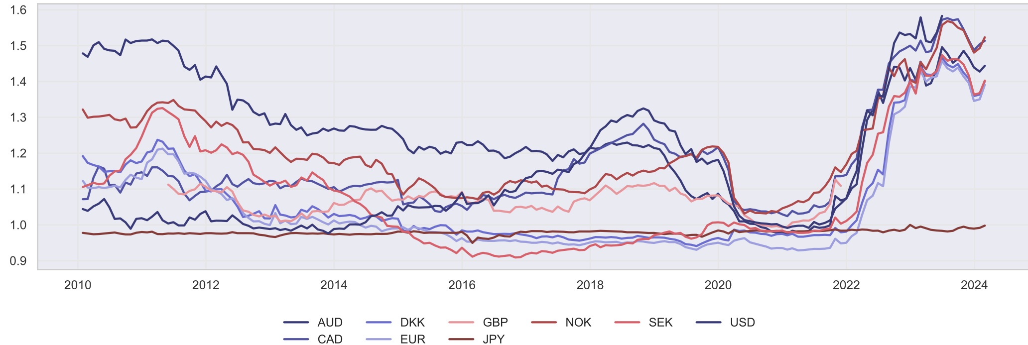
Volatility sigma1(z)
