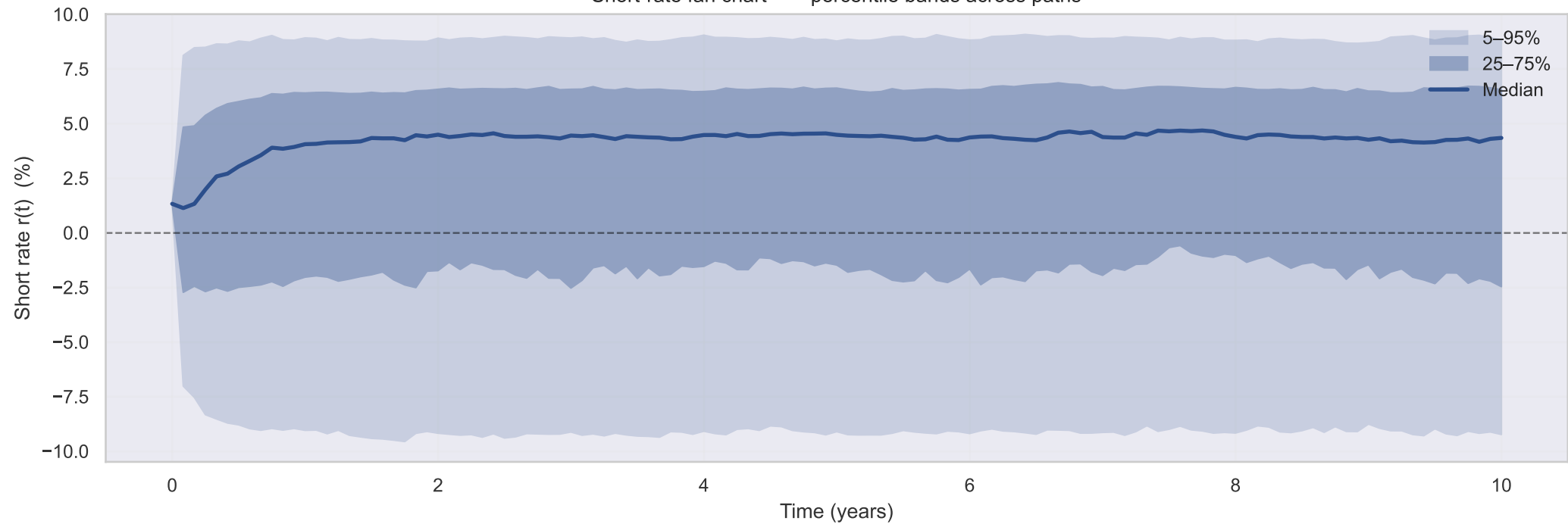
Short-rate fan chart — percentile bands across paths
