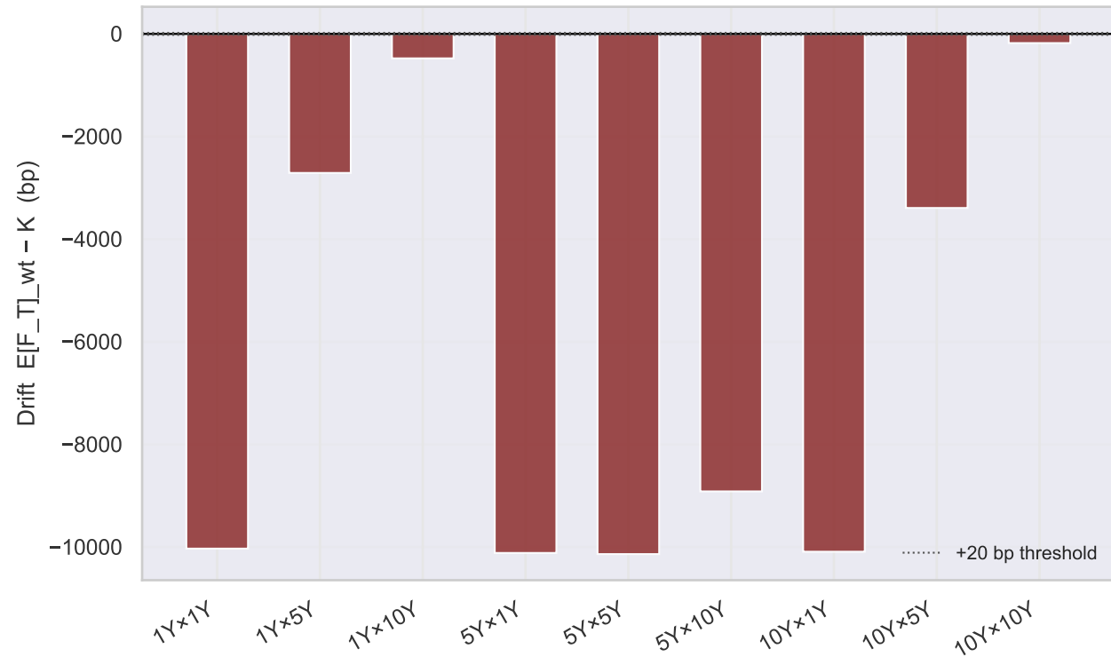
Annuity-weighted drift per (expiry \times tenor) Blue = paths above strike, Red = below
