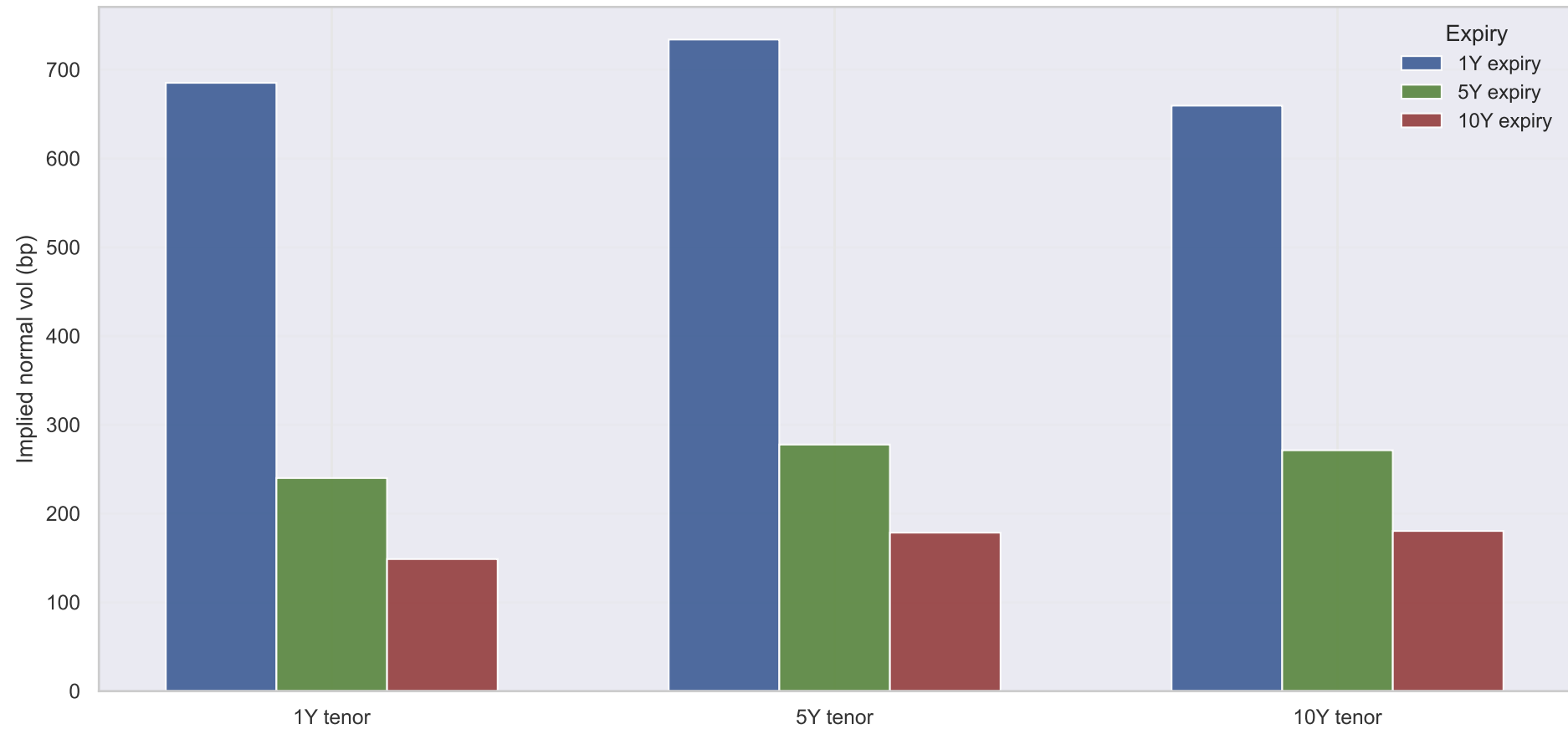
Model-implied ATM normal vol — grouped by option expiry
