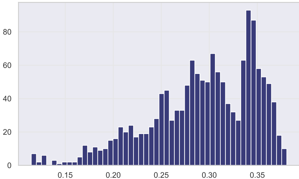
Histogram of \mu_3
