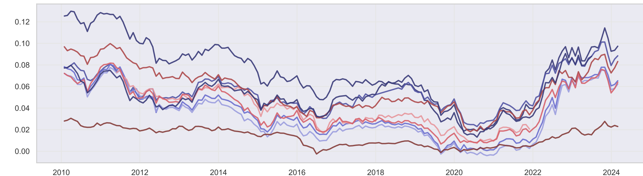
Latent factors for 3-factor model
