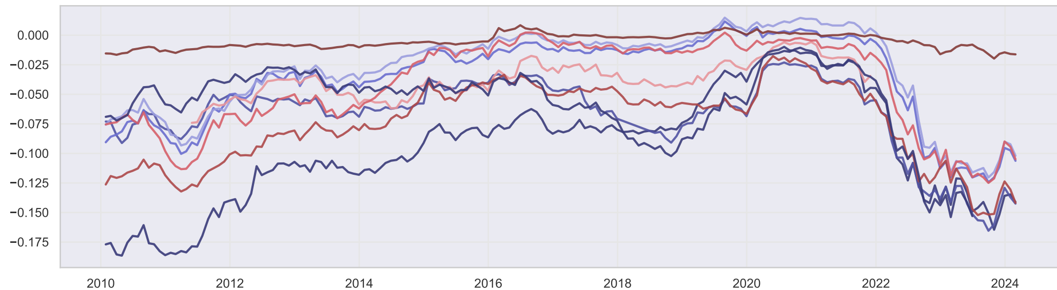
Latent factors for 2-factor model
