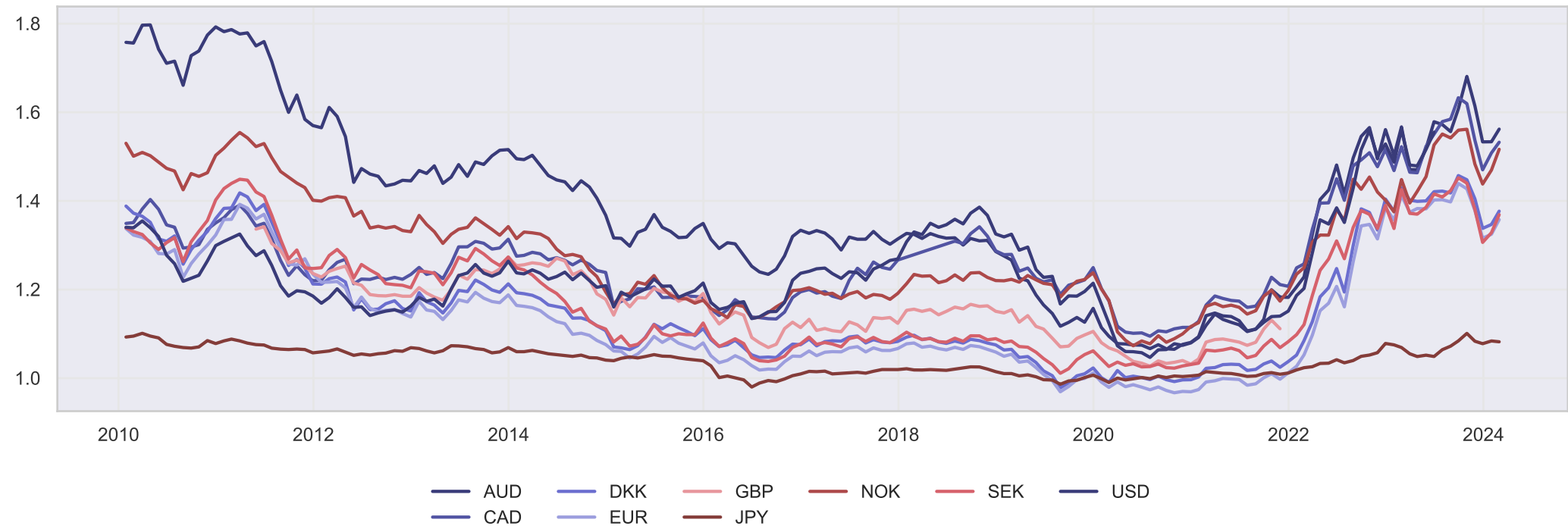
Volatility sigma3(z)
