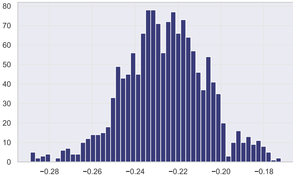
Histogram of \mu_1
