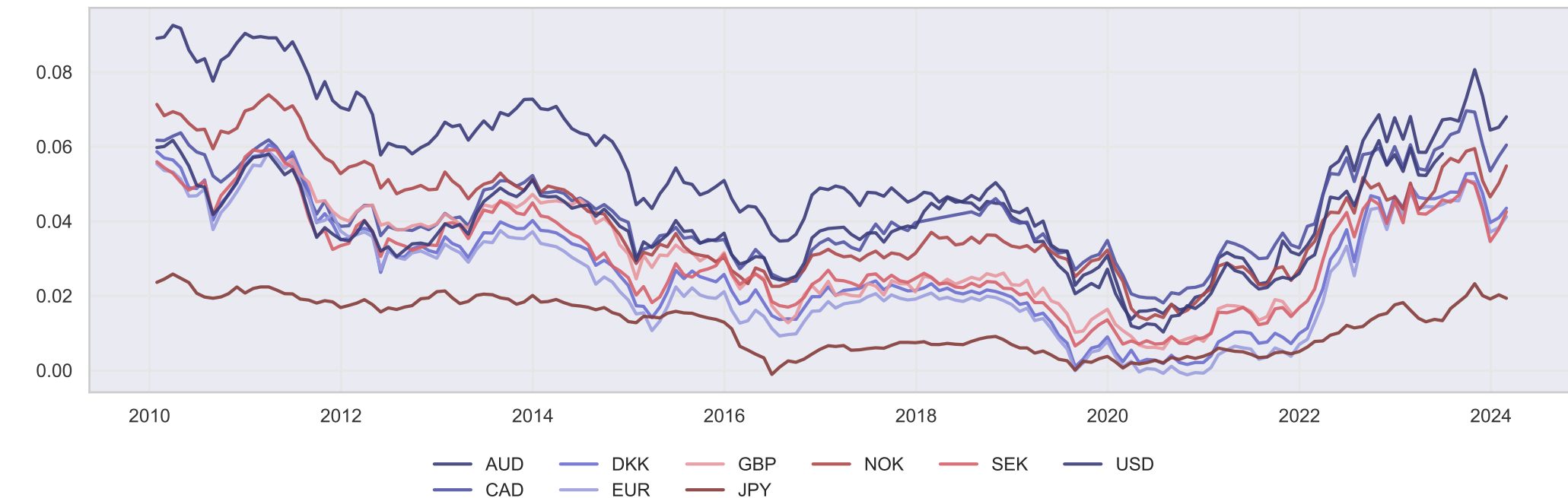
Latent factors for 2-factor model
