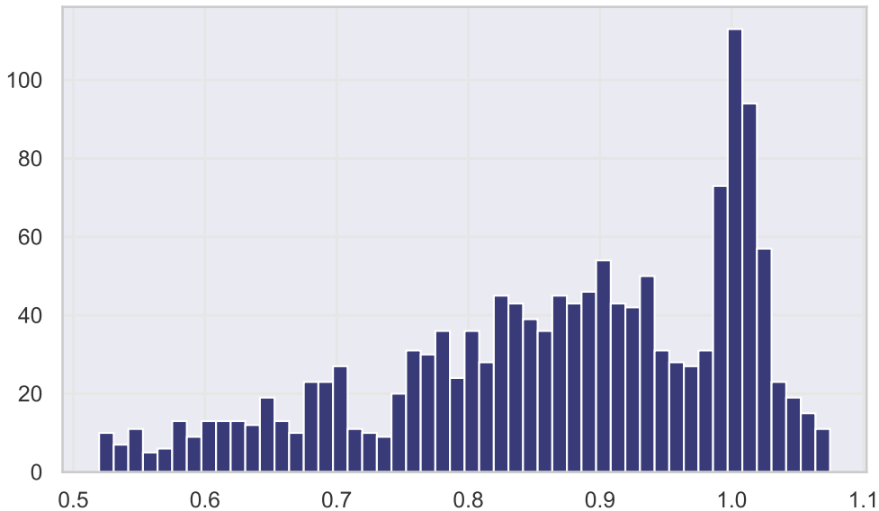
Histogram of sigma2
