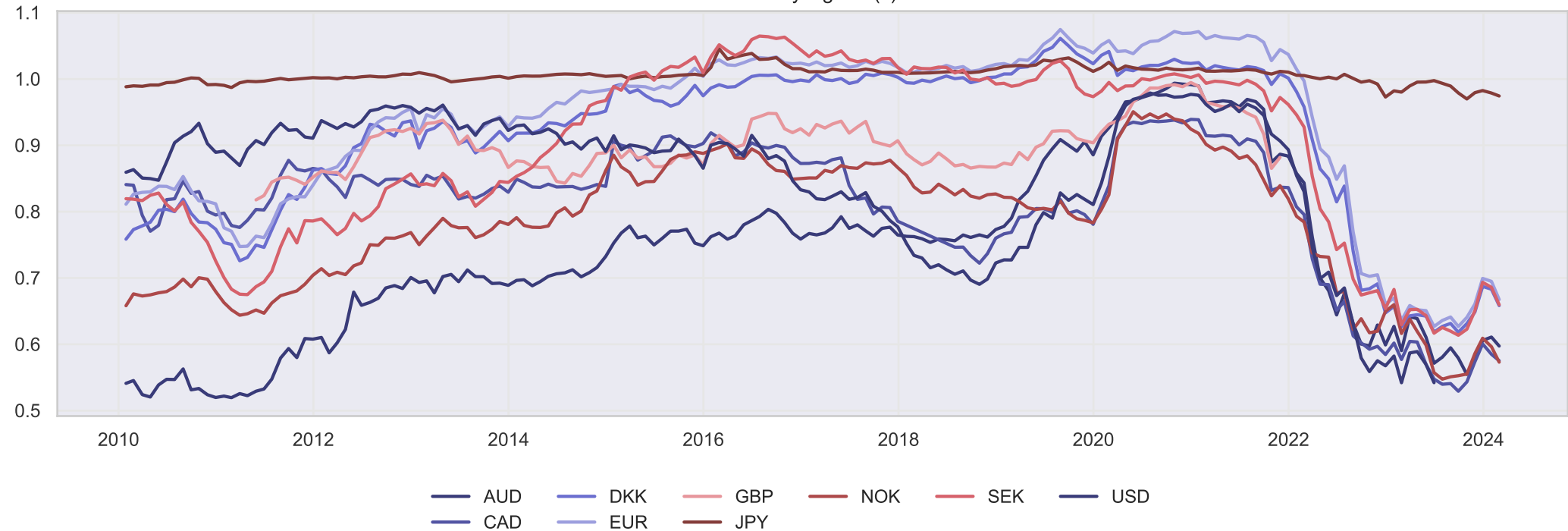
Volatility \sigma^2(z)
