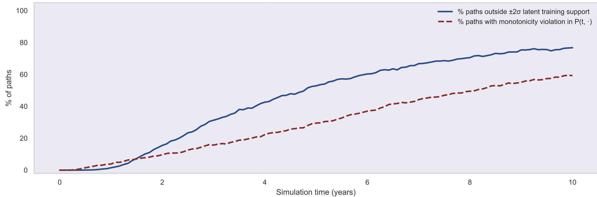
Latent extrapolation and curve violations rise together
