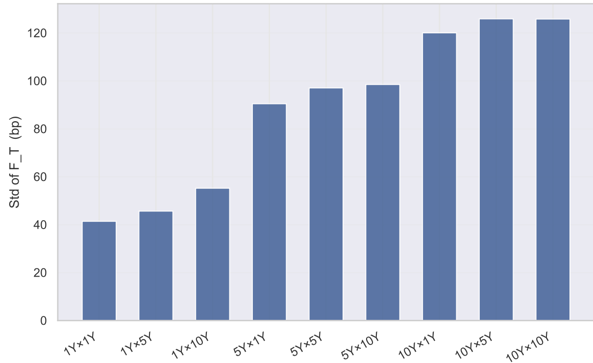
Dispersion of realized swap rate at expiry Captures the vol the model generates
