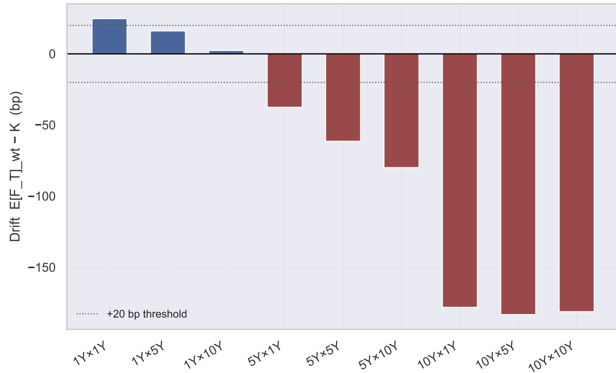
Annuity-weighted drift per (expiry \times tenor) Blue = paths above strike, Red = below
