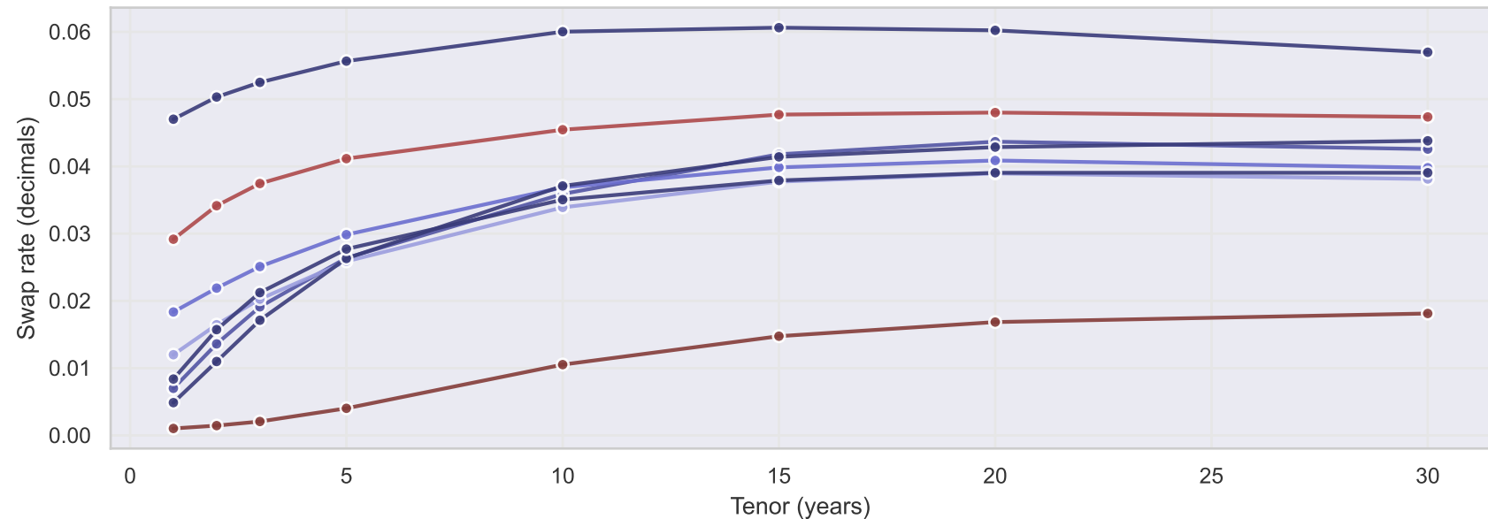
Observed swap curves on 2010-01-29
