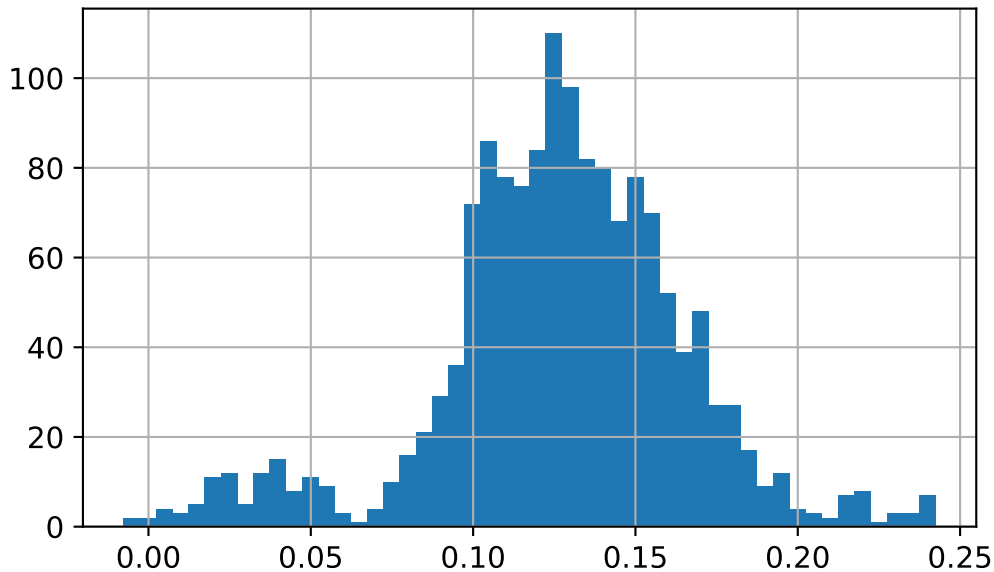
Histogram of mu1
