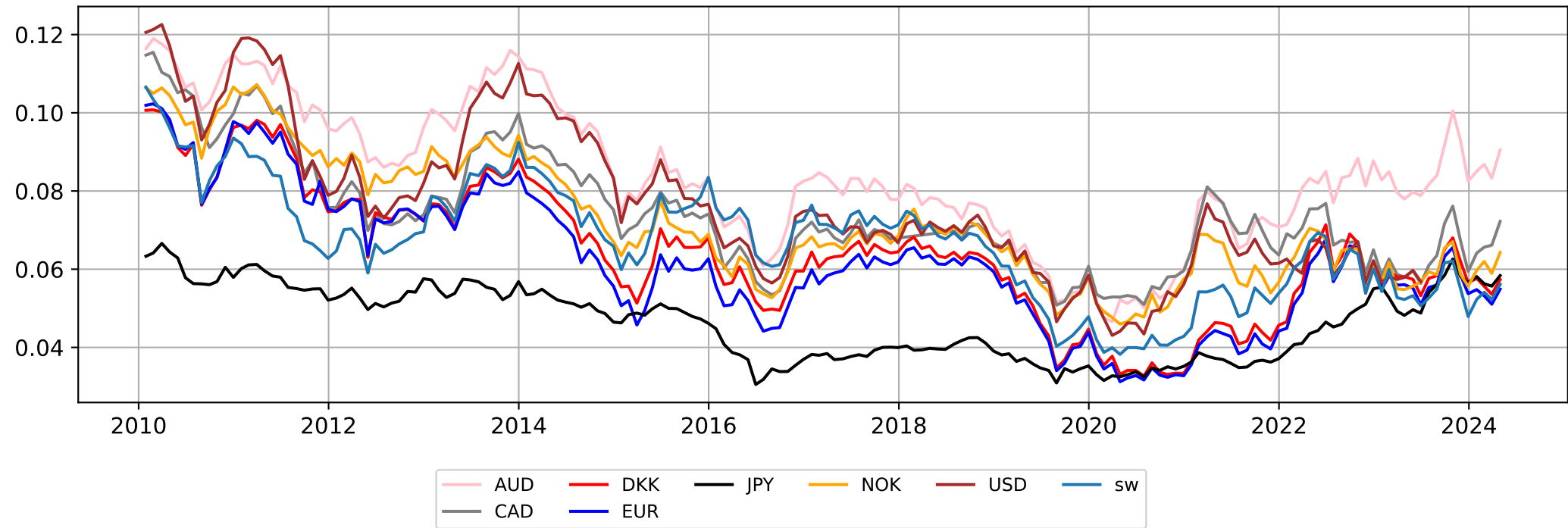
Drift \mu_2(z)
