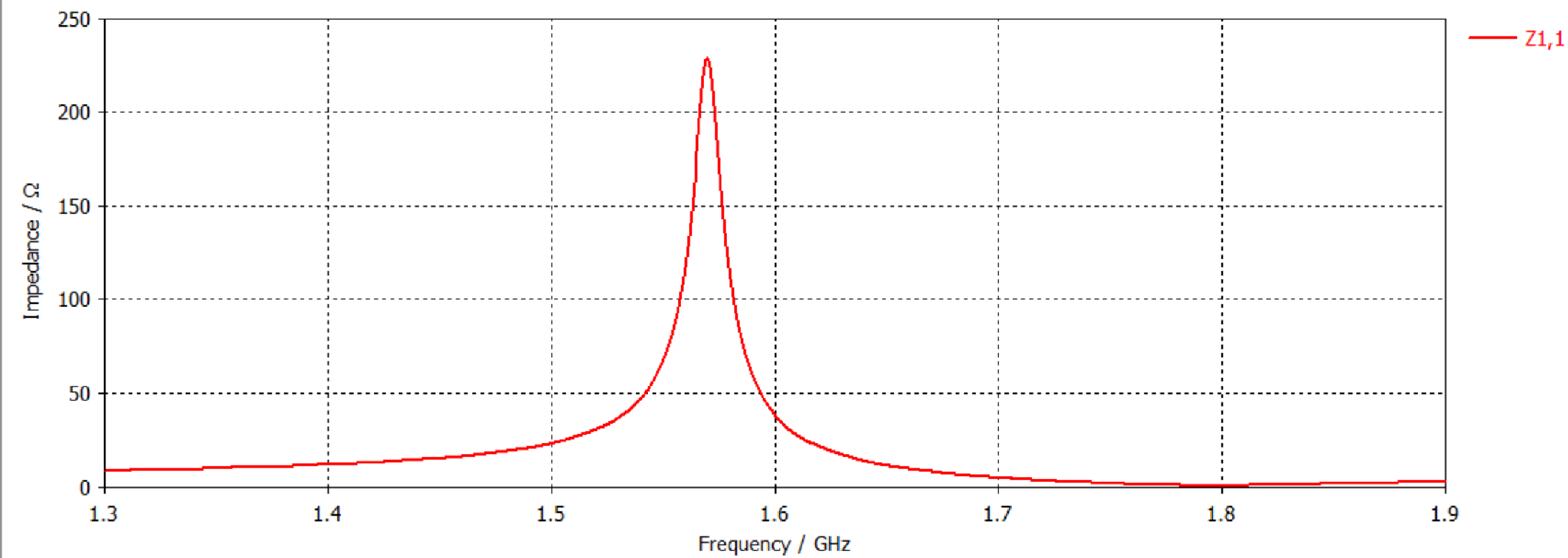
Z-Parameters [Magnitude]
