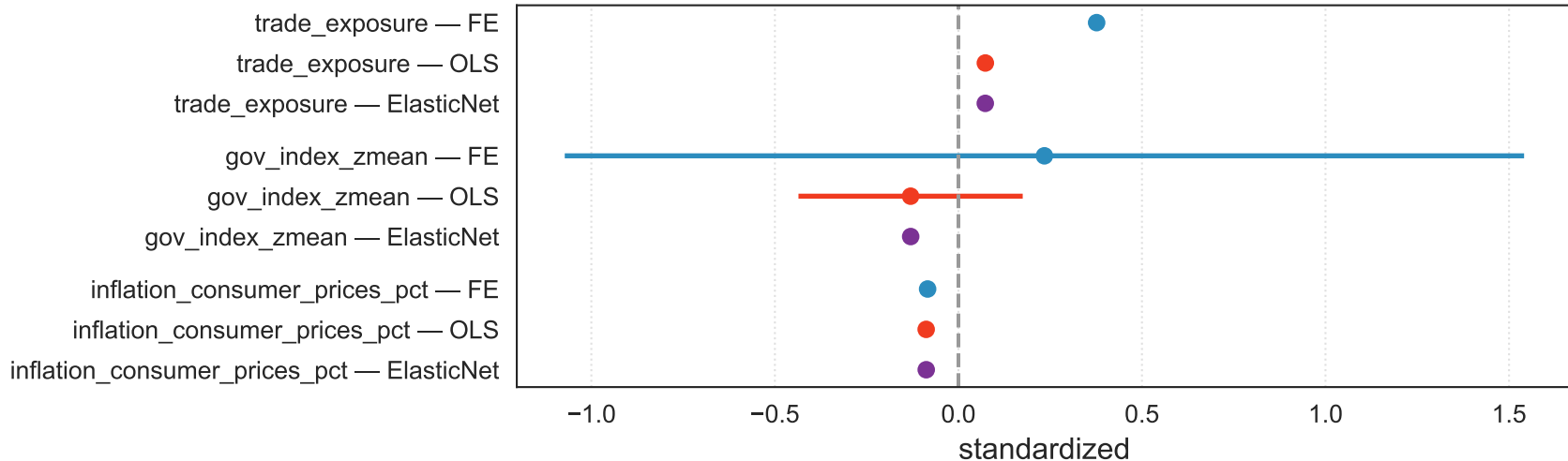
Standardized effects ( \sigma of target) by model
