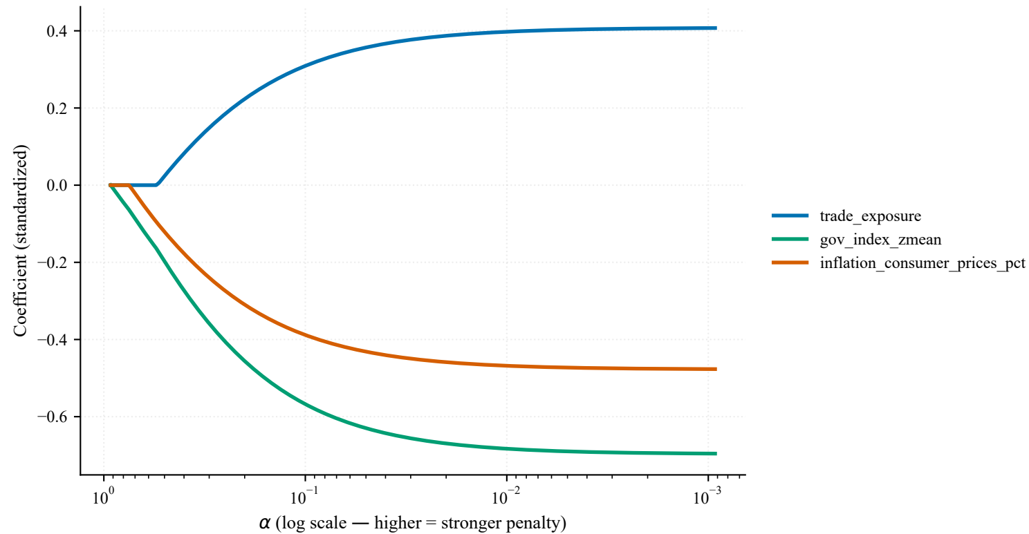
ElasticNet coefficient path (l1_ratio=0.5)
